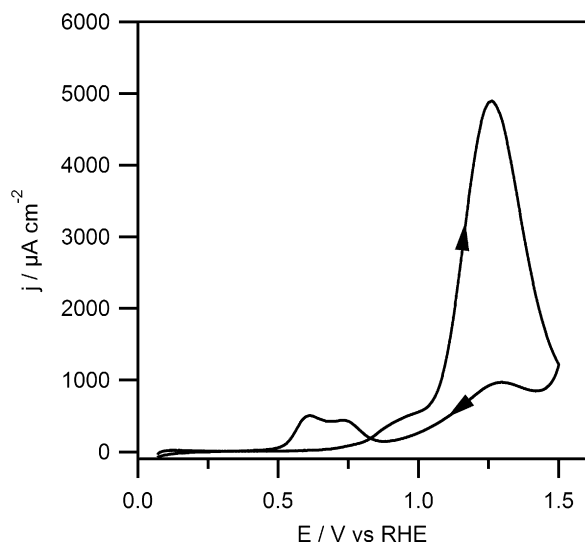
Fig. 10. Cyclic voltammogram for the oxidation of 0.5 M acetaldehyde in 0.1 M \text{HClO}_4 on polycrystalline platinum. The voltammogram is recorded at 50 \text{ mV s}^{-1} . The arrows indicate the scan directions.
