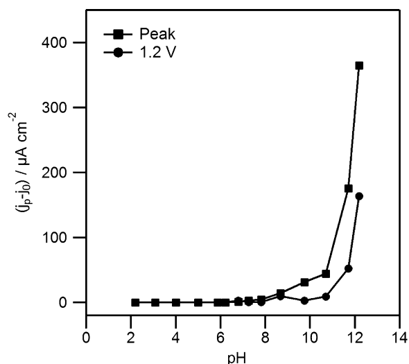
Fig. 13. Corrected peak currents and currents at 1.2 V (see text) obtained from the cyclic voltammograms for the oxidation of 0.5 M ethanol in 0.1 M phosphate buffers of pH 2–12.
