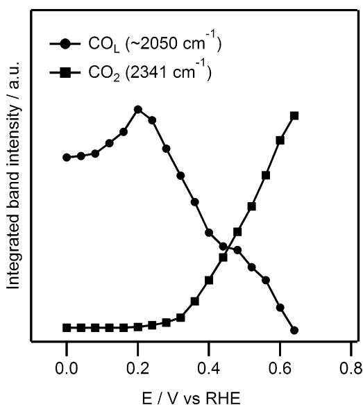
Fig. 3. Integrated band intensities for the bands at ~2050 cm -1 (CO L ) and 2341 cm -1 (CO 2 ) measured in FTIR experiments for the oxidation of ethanol in 0.1 M HClO 4 on platinum.
