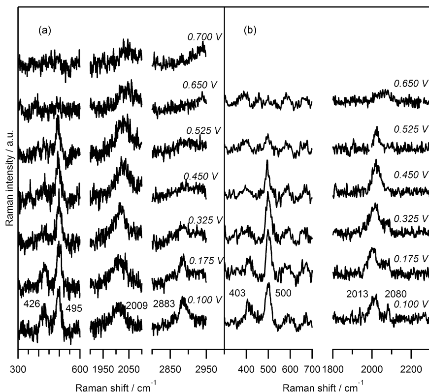
Fig. 4. Surface enhanced Raman spectra of (a) ethanol and (b) deuterated ethanol (ethanol- d_6 ) dissociation products on a Pt-film electrode in 0.1 M \text{HClO}_4 recorded at the indicated potentials. Reproduced with permission from Ref. [21].
