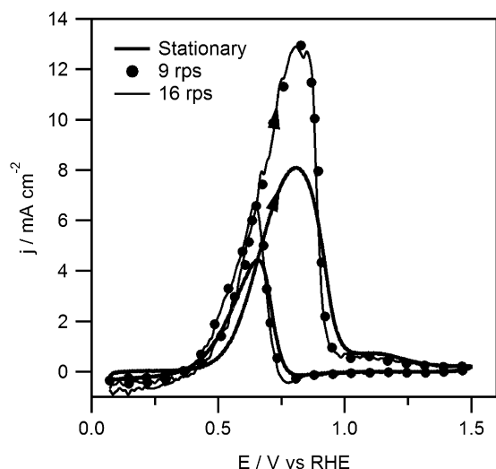
Fig. 8. Cyclic voltammograms for the oxidation of 0.5 M ethanol in 0.1 M phosphate buffers of pH 11.32 recorded under stationary conditions and at rotation rates of 9 and 16 rotations per second. The voltammograms are recorded at 50 \text{ mV s}^{-1} . The arrows indicate the scan directions.
