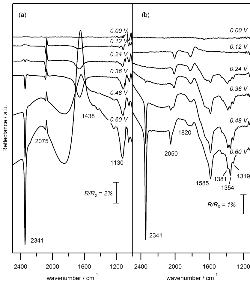
Fig. 2. In situ FTIR spectra for the electro-oxidation of ethanol on platinum in (a) 0.1 M \text{HClO}_4 and (b) 0.1 M \text{NaOH} . The reference spectrum was taken at 0.0 V. The sample spectra are measured during a voltammetric sweep at 10 \text{ mV s}^{-1} at the indicated potentials.
