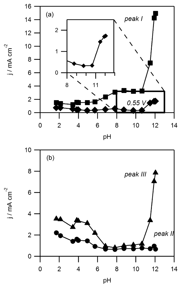
Fig. 7. Peak currents obtained from voltammograms for the oxidation of 0.5 M ethanol in 0.1 M phosphate buffers of pH 2–12. Peaks I and II refer to the first peak (ca. 0.9 V) and second peak (ca. 1.3 V) in the positive sweep, respectively, while peak III refers to the peak in the negative sweep. In addition, the currents obtained from the voltammograms at a fixed potential of 0.55 V in the positive sweep are also included.
