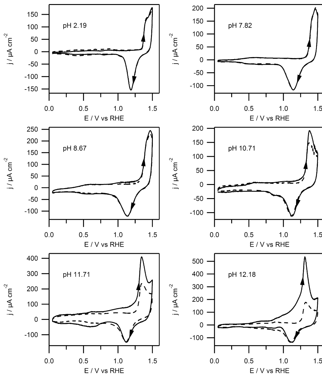
Fig. 12. Cyclic voltammograms for polycrystalline gold in 0.1 M phosphate buffers (pH 2–12) in the absence (dotted lines) and in the presence of 0.5 M ethanol (solid lines). The voltammograms are recorded at 50 \text{ mV s}^{-1} . The arrows indicate the scan direction.
