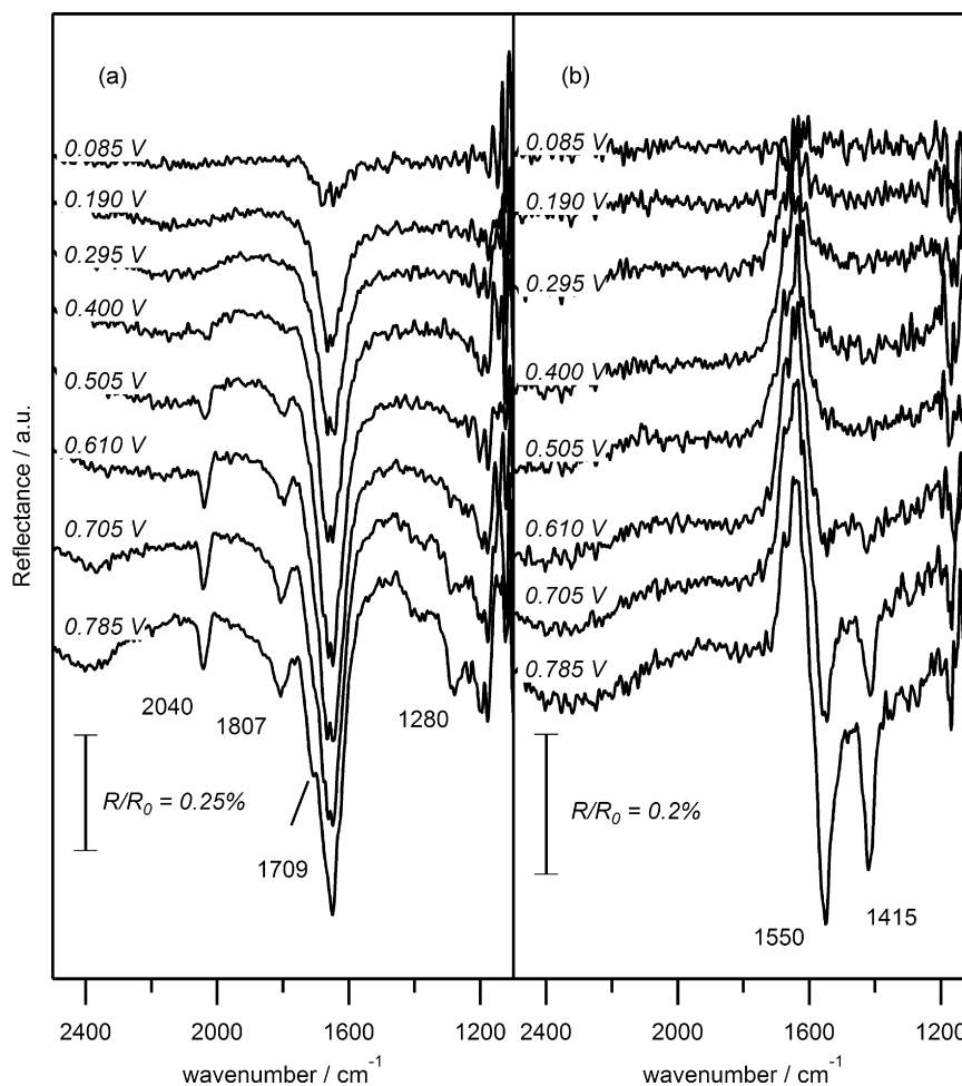
Fig. 9. In situ FTIR spectra for the electro-oxidation of ethanol on platinum in a 0.1 \text{ M} phosphate buffer of (a) pH 2 and (b) pH 12. The reference spectrum was taken at 0.0 \text{ V} . The sample spectra are measured during a voltammetric sweep at 10 \text{ mV s}^{-1} at the indicated potentials.
