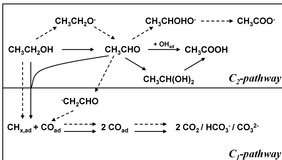
Scheme 1. Proposed reaction mechanism for the ethanol electro-oxidation reaction. Solid arrows denote the mechanism at low electrolyte pH, while dashed arrows denote the mechanism at high electrolyte pH.
