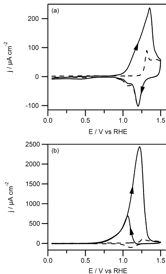
Fig. 11. Cyclic voltammograms for polycrystalline gold in (a) 0.1 M \text{HClO}_4 and (b) 0.1 M \text{NaOH} in the absence (dotted lines) and in the presence of 0.5 M ethanol (solid lines). The voltammograms are recorded at 50 \text{ mV s}^{-1} . The arrows indicate the scan direction.
