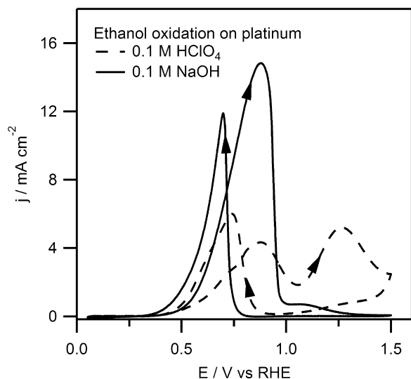
Fig. 1. Cyclic voltammograms (first cycles) for the oxidation of 0.5 M ethanol in 0.1 M \text{HClO}_4 and 0.1 M \text{NaOH} on polycrystalline platinum. The voltammograms are recorded at 50 \text{ mV s}^{-1} . The arrows indicate the scan direction.
