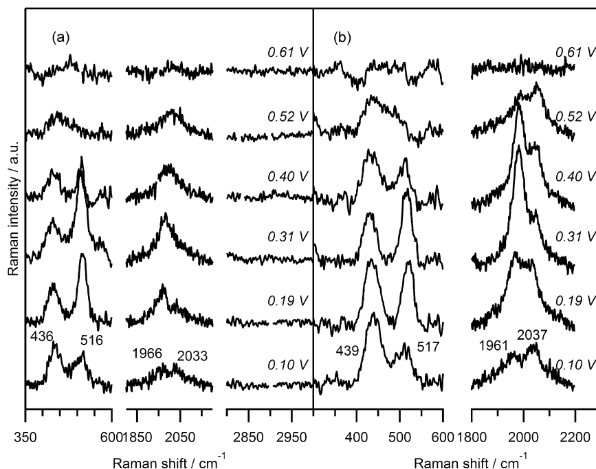
Fig. 5. Surface enhanced Raman spectra of (a) ethanol and (b) deuterated ethanol (ethanol- d_6 ) dissociation products on a Pt-film electrode in 0.1 M NaOH recorded at the indicated potentials. Reproduced with permission from Ref. [33].
